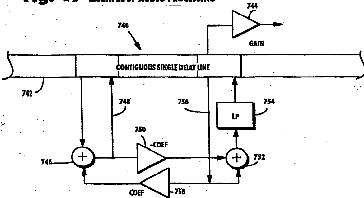
Fig. 17 EXAMPLE SP AUDIO PROCESSING
